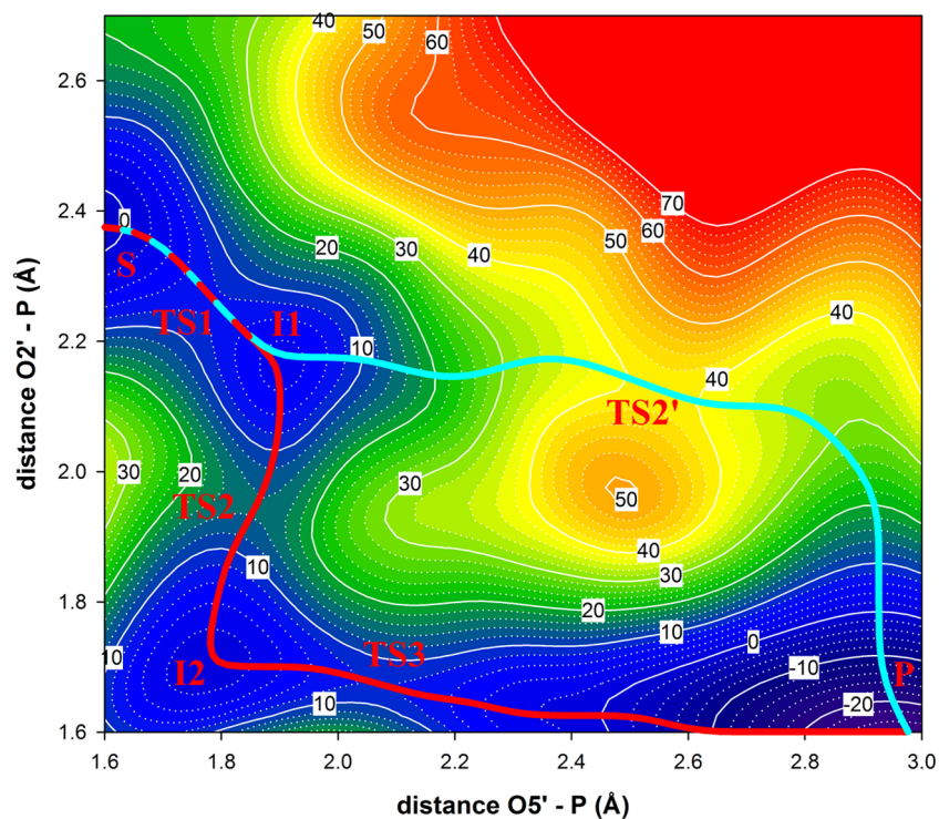
Figure 4. Free-energy surface for the RNase A reaction obtained using the FIREBALL/AMBER system (in kcal/mol). Axes represent the reaction coordinates (distances O2'-P and O5'-P , respectively). The two possible reaction trajectories are indicated: dissociative S_N1 pathway in cyan and associative S_N2 pathway in red. The positions of substrate (S), transition states (TS), intermediate states (I), and reaction product (P) in both pathways are indicated.
