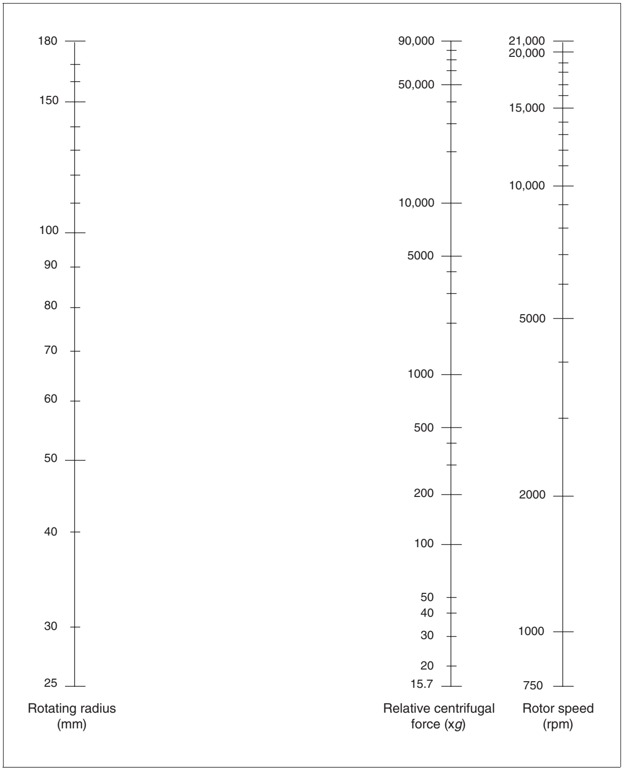
Figure A.2B.1 Nomogram for conversion of relative centrifugal force to rotor speed in low-speed centrifuge runs. To determine an unknown value in a given column, align ruler through known values in the other two columns. Desired value is found at the intersection of the ruler with the column of interest. For faster centrifugations, use Figure A.2B.2. A more precise conversion can be obtained using the equation at the beginning of this appendix. See Table A.2B.1 for rotating radii of commonly used rotors.
