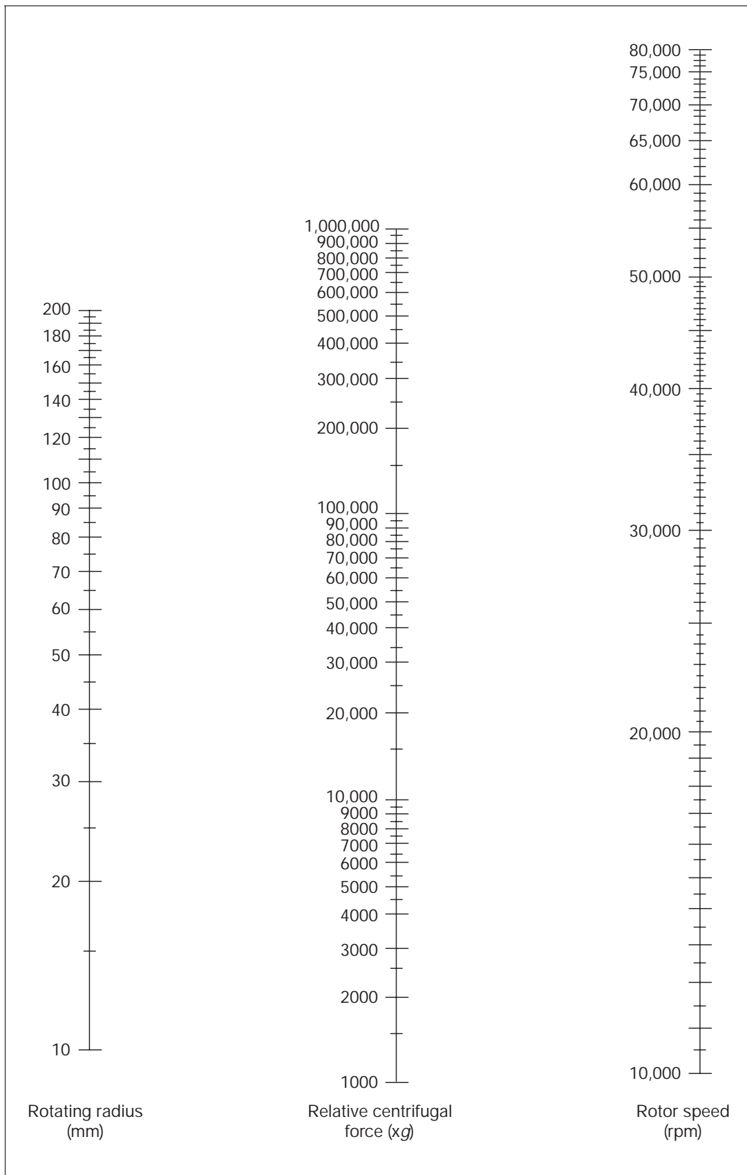
Figure A.2B.2 Nomogram for conversion of relative centrifugal force to rotor speed in high-speed centrifuge runs. For slower centrifugations and instructions for using the nomogram, use Figure A.2B.1. A more precise conversion can be obtained using the equation at the beginning of this appendix. See Table A.2B.1 for rotating radii of commonly used rotors.
